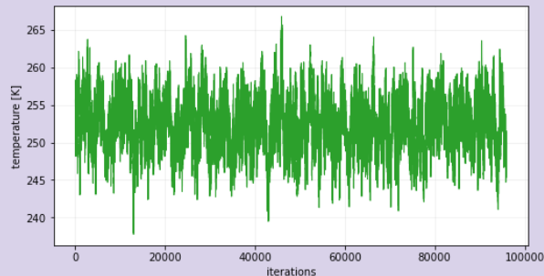
Teff Post Burn-In
