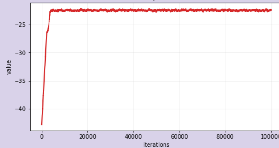
alpha Post Burn-In
