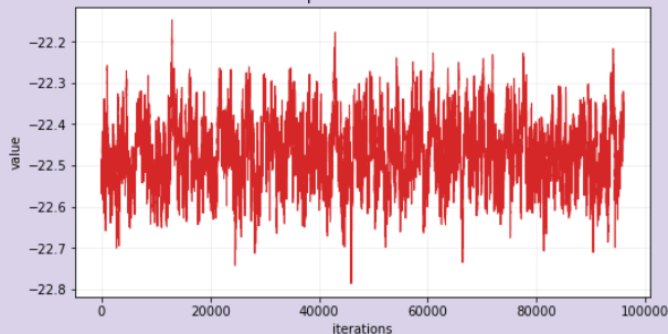
alpha Post Burn-In
