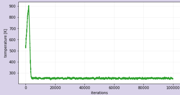
Teff Post Burn-In
